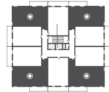
Eleventh floor
