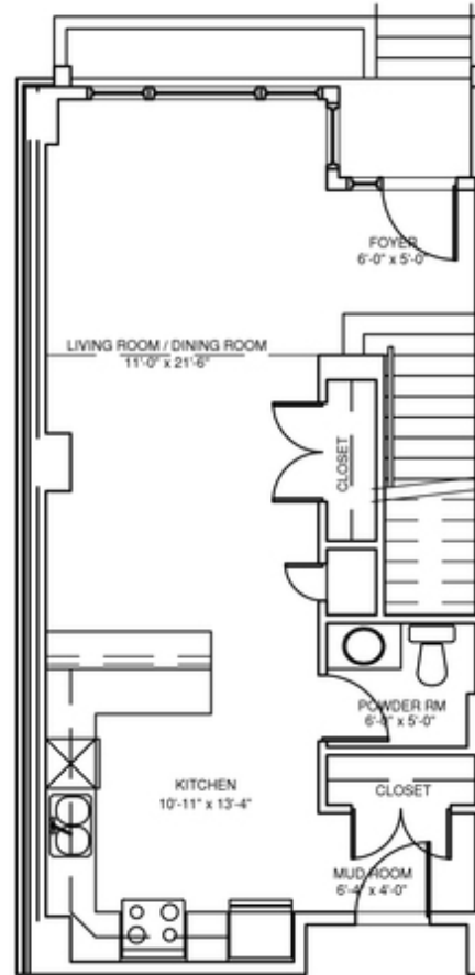
1ST FLOOR
