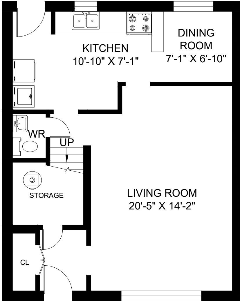
1ST FLOOR
