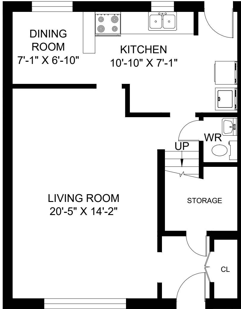
1ST FLOOR
