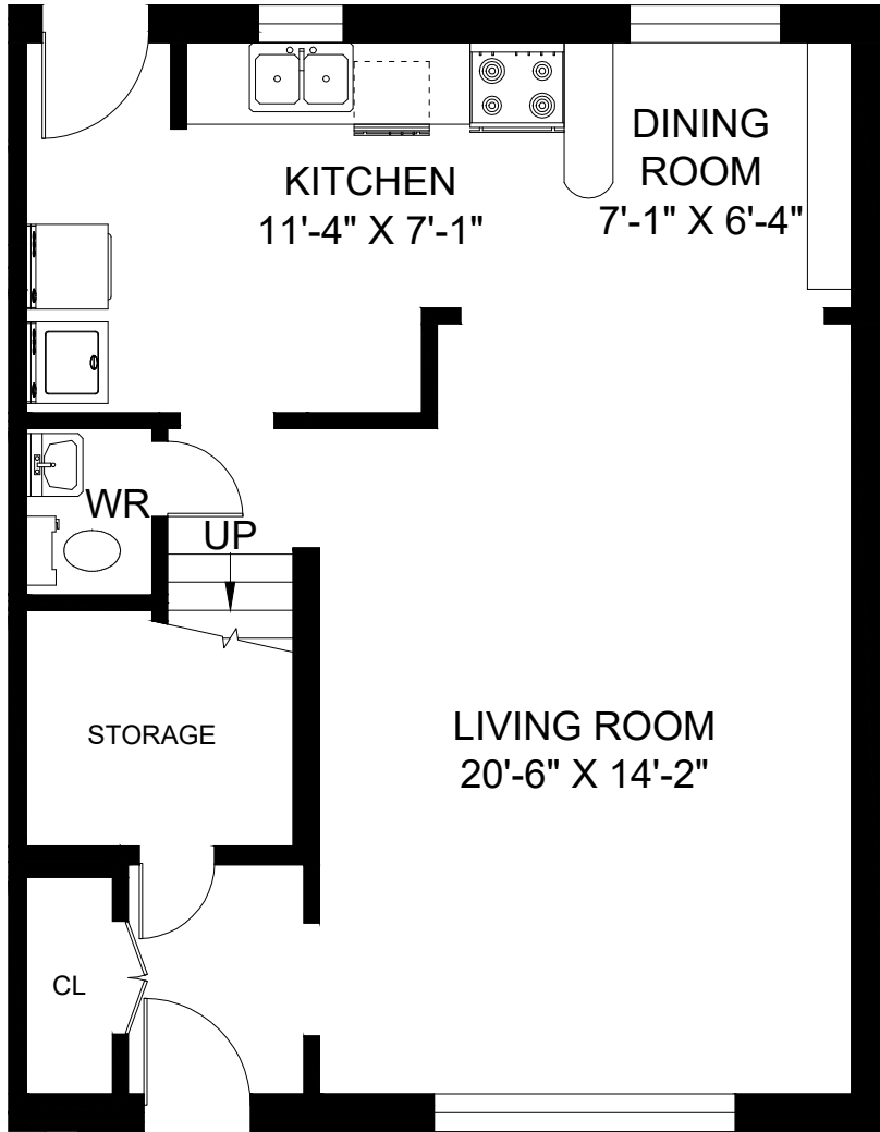
1ST FLOOR
